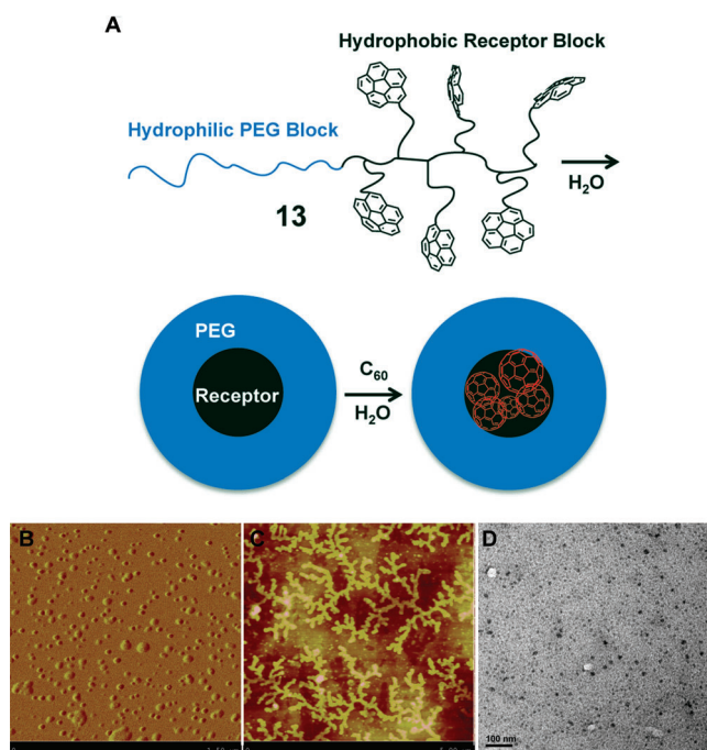
Figure 4. A) Schematic representation of micelle formation and C_{60} encapsulation by copolymer 13 in water. B,C) AFM images of the nanostructures formed by 13 + C_{60} in water on mica (B) and on HOPG (C). D) TEM image of 13 + C_{60} in water on a carbon-coated copper grid (scale bar: 100 nm).
